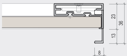
96 mm handle horizontal section
