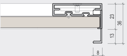
150 mm handle horizontal section
