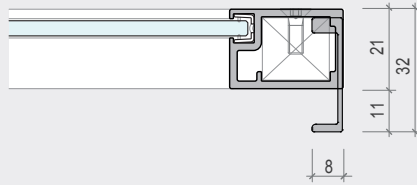
150 mm handle horizontal section
