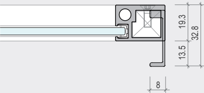
96 mm handle horizontal section
